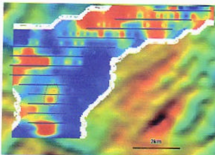
Image of CH8 ground TEM over magnetics, interpreted bedrock conductor highlighted (purple dashed line) the other conductive signatures are the result of near surface effects.
